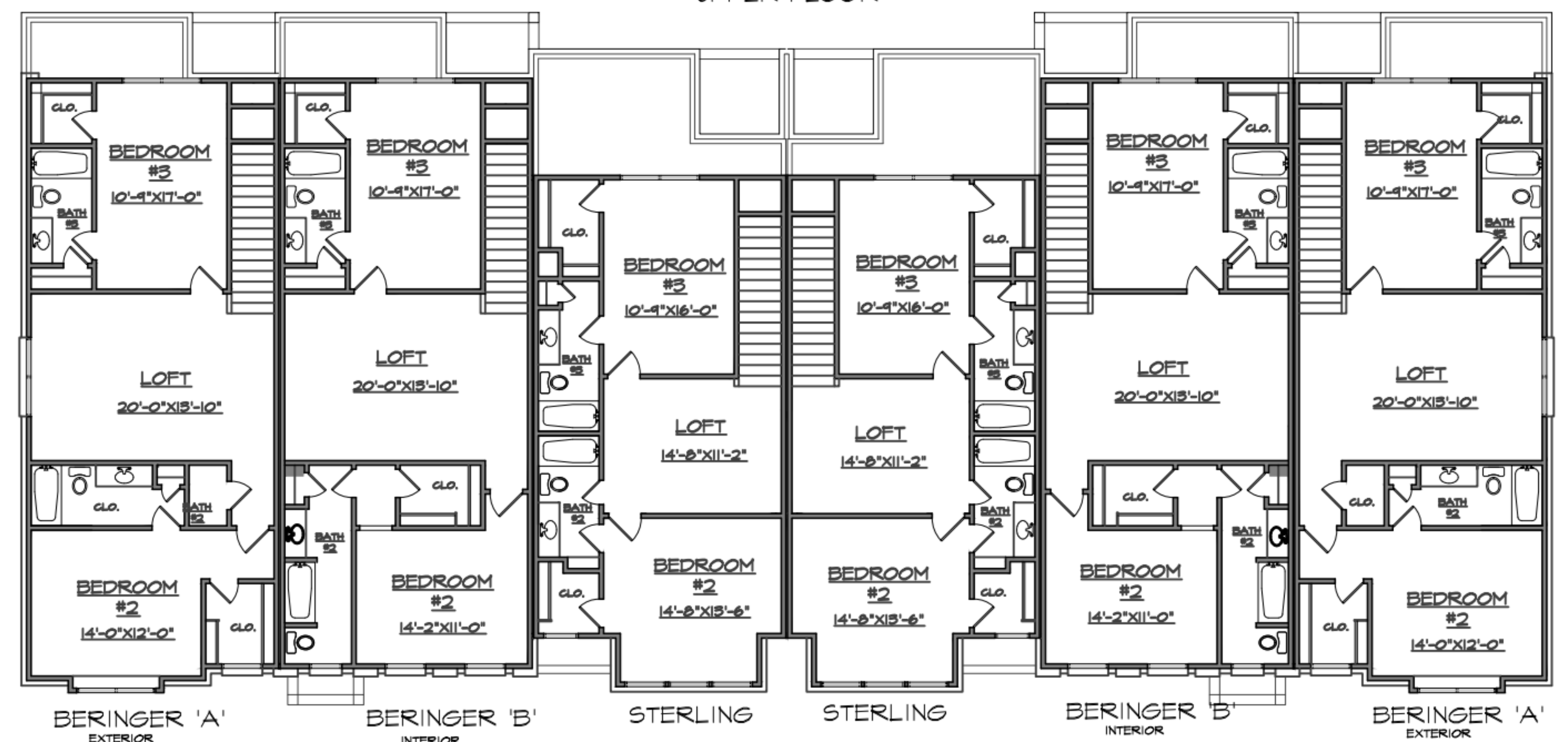
The Reserve At Oxford Farms UPPER FLOOR
